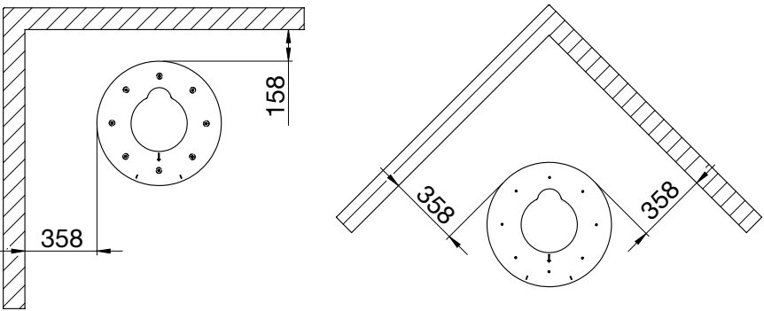
Safety distances for placement of the optional leveling base.
